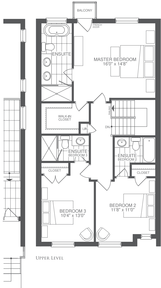
UPPER LEVEL FOR TH-3 END UNIT (2563 SQ.FT.)
