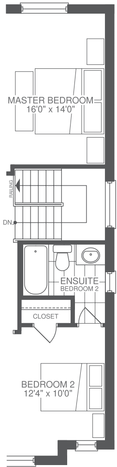
UPPER LEVEL FOR TH-3 END UNIT (2563 SQ.FT.)
